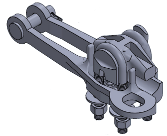
Aluminum Straight Line Clamp ASOSLC Series
