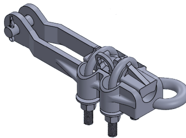
Aluminum Straight Line Clamp ASLC Series
