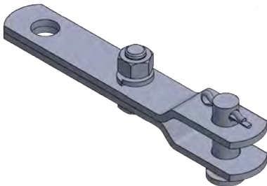
Extension Links Clevis-Eye ELS-CE Series
