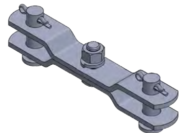
Extension Links Clevis-Clevis ELS-CC Series
